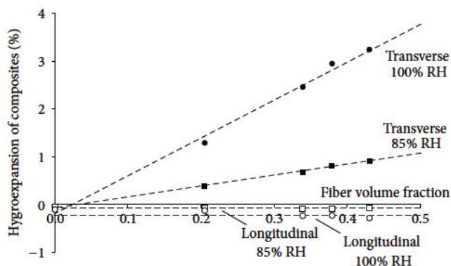
FIGURE 8: Hydroexpansion of unidirectional hemp fiber/polyethylene terephthalate composites as function of the fiber volume fraction. Hydroexpansion was measured in the longitudinal and transverse directions, and at the humidities of 85 and 100% RH, with respect to a reference humidity of 65% RH. Lines are calculated by micromechanical models. Modified from [80].
