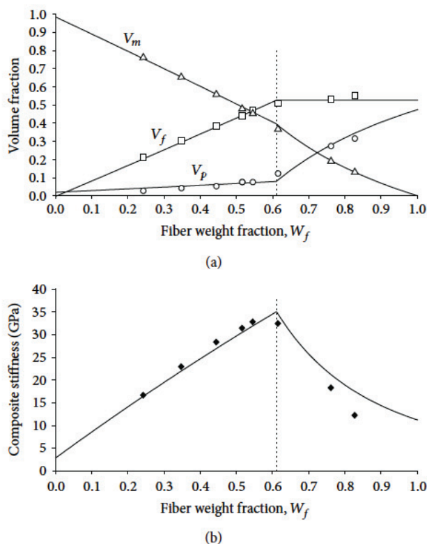
FIGURE 7: Experimental data and model predictions of (a) volumetric composition ( V_f , V_m , and V_p ) and (b) stiffness as a function of the fiber weight fraction of unidirectional flax fiber/polyethylene terephthalate composites. Vertical dotted lines indicate the transition fiber weight fraction. Data from [75].
