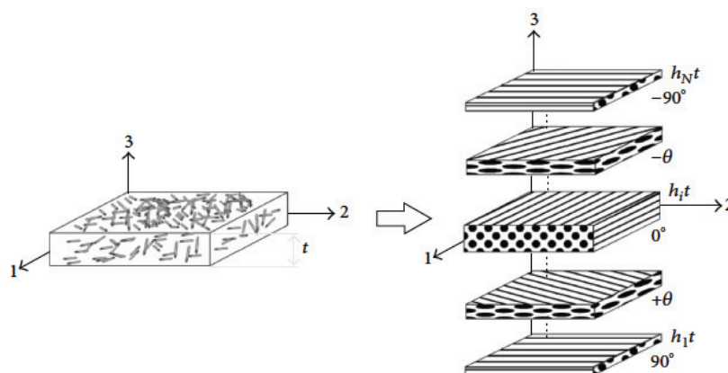
FIGURE 4: Schematic illustration of a laminate analogy for randomly oriented cellulose fiber composites.
